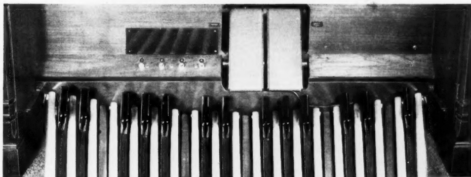
The detachable pedal unit consists of a 32-note console and radiating clavier. It is built according to A. G. O. standard dimensions. The sharp keys are molded Bakelite and the natural keys maple with a wear-resisting finish. The four toe pistons to the left of the expression pedals enable the organist to use any desired pedal quality. The two expression pedals independently affect their respective manuals. Each operates over the wide range for which the Hammond is noted—the most effective dynamic control known to music.
